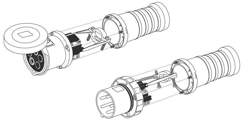
63 - 125 А, IP44
